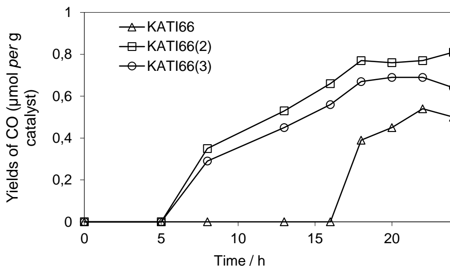
Fig. 7 Time dependence of the hydrogen (A) and the carbon monoxide (B) yields over the kaolinite/ TiO 2 catalysts calcined for different calcination time.
